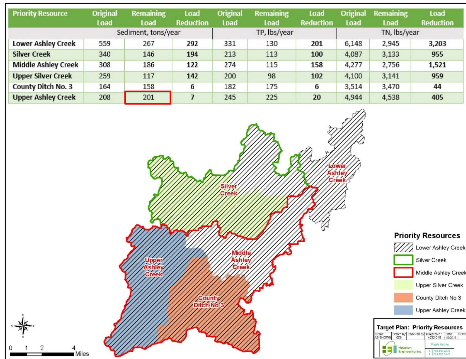
Figure 22. Sediment, TP, and TN reductions based upon Scenario 2 for Ashely Creek.
